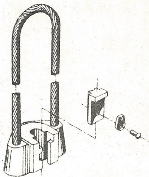
BABBITTED TYPE
