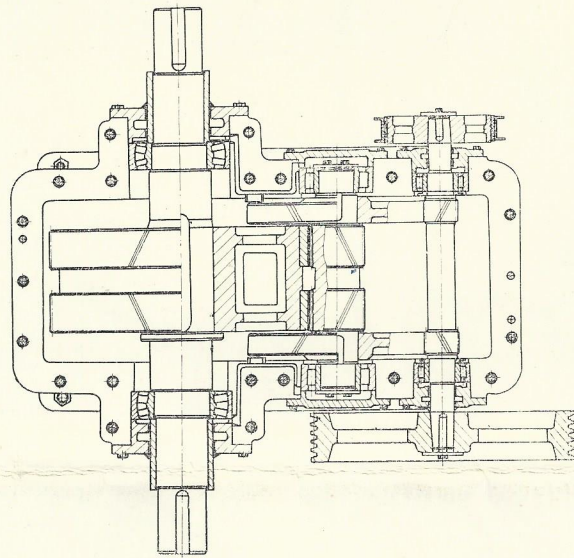
园弧齿人字齿轮减速器 Circular arc tooth herringbone gear reducer
